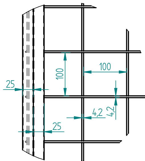
DETAIL A
